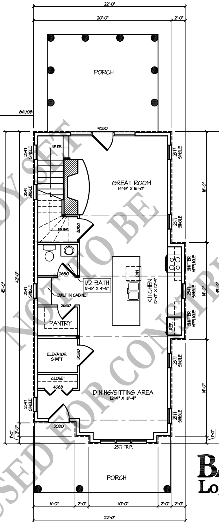
1st FLOOR PLAN (884 S.F.)
